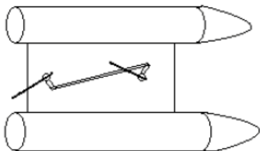
View from bottom of boat on dual rudder system.
