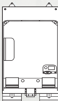
Angler - Floor Plan Includes steering console, 2 rear seats and cushioned side seat with integrated livewell
